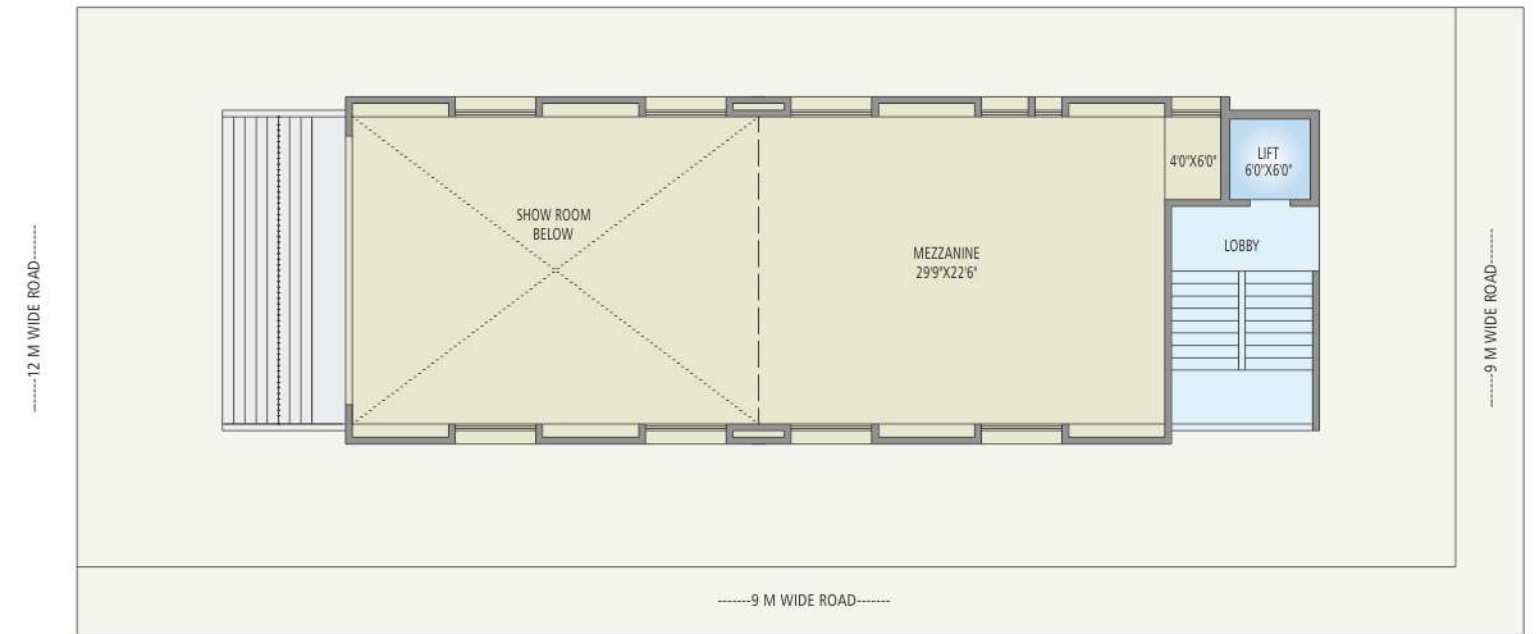
Mezzanine Floor Plan
