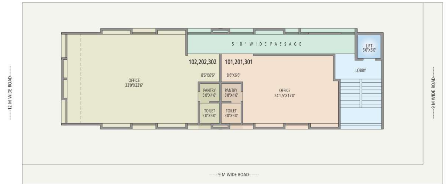
Typical 1st, 2nd, 3rd Floor Plan
